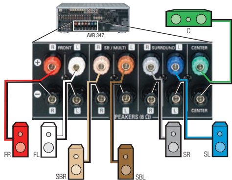
Figure 17 – Speaker Connections
